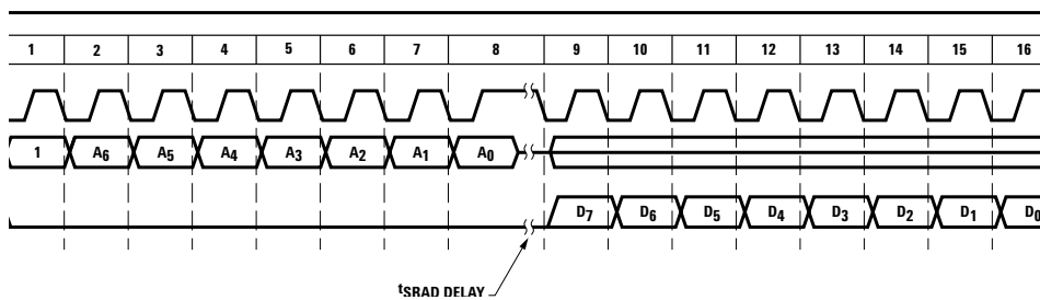
Figure 13. Read operation
