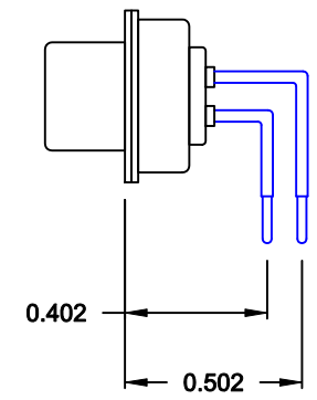
SIGNAL CONTACTS
