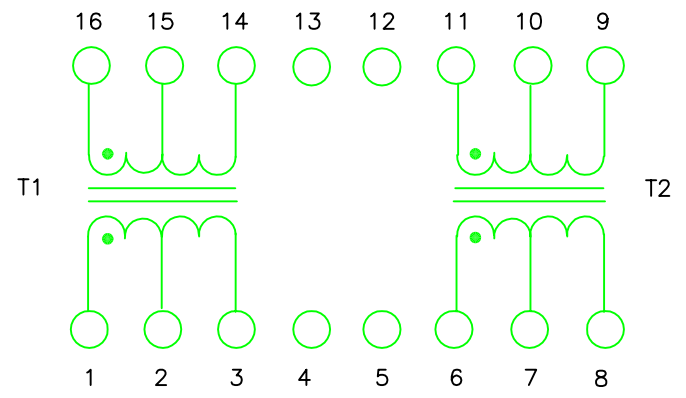
SCHEMATIC
