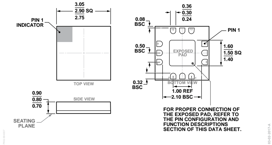
Figure 86. 12-Terminal Ceramic Leadless Chip Carrier (LCC) (E-12-4) Dimensions shown in millimeters
