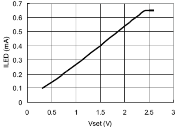
12. I_{LED} VS V_{SET} ( V_{IN} = 16\text{V} , 3 LEDs, 100\mu\text{H} , R_s = 0.3\Omega )
