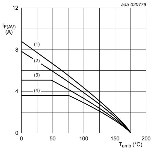
Ceramic PCB, \text{Al}_2\text{O}_3 , standard footprint T_j = 175\text{ }^\circ\text{C} (1) \delta = 1 (DC) (2) \delta = 0.5 ; f = 20\text{ kHz} (3) \delta = 0.2 ; f = 20\text{ kHz} (4) \delta = 0.1 ; f = 20\text{ kHz}
