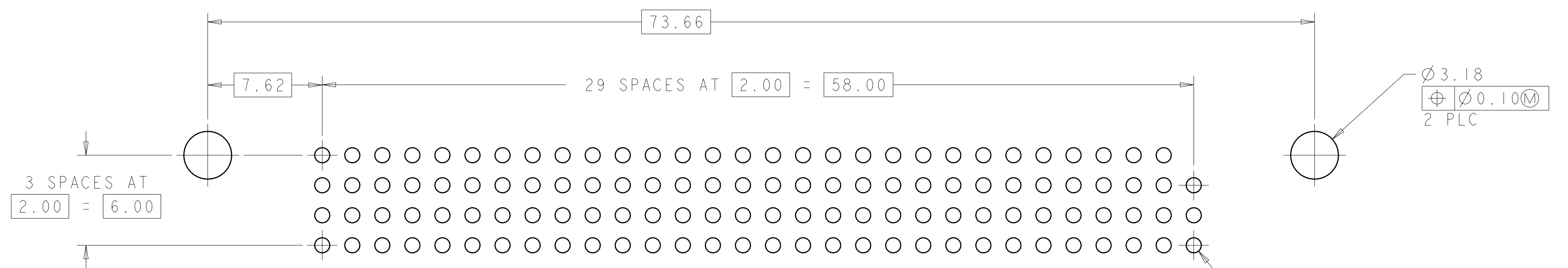
RECOMMENDED PCB LAYOUT FOR 1375965-3 & -6
