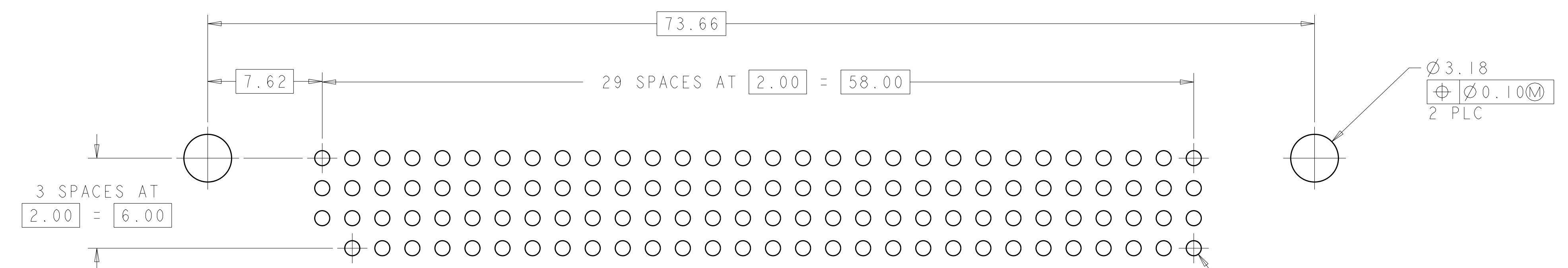
RECOMMENDED PCB LAYOUT FOR 1375965-2 & -5
