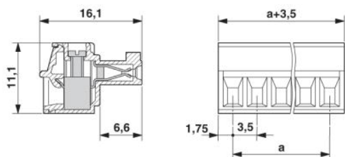
Dimensioned drawing
