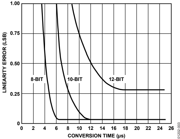
Figure 3. Linearity Error vs. Conversion Time (Normalized)
