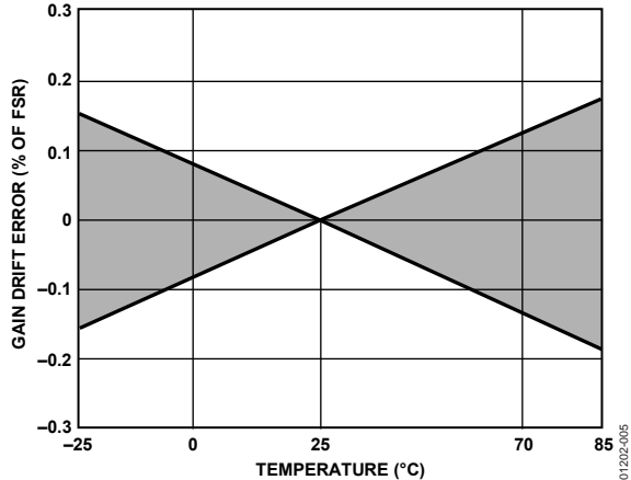
Figure 4. Gain Drift Error vs. Temperature
