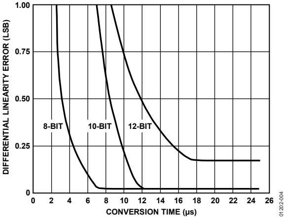
Figure 5. Differential Linearity Error vs. Conversion Time (Normalized)
