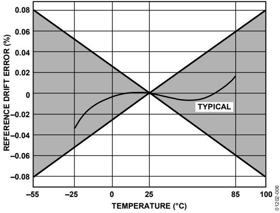
Figure 6. Reference Drift, Error vs. Temperature
