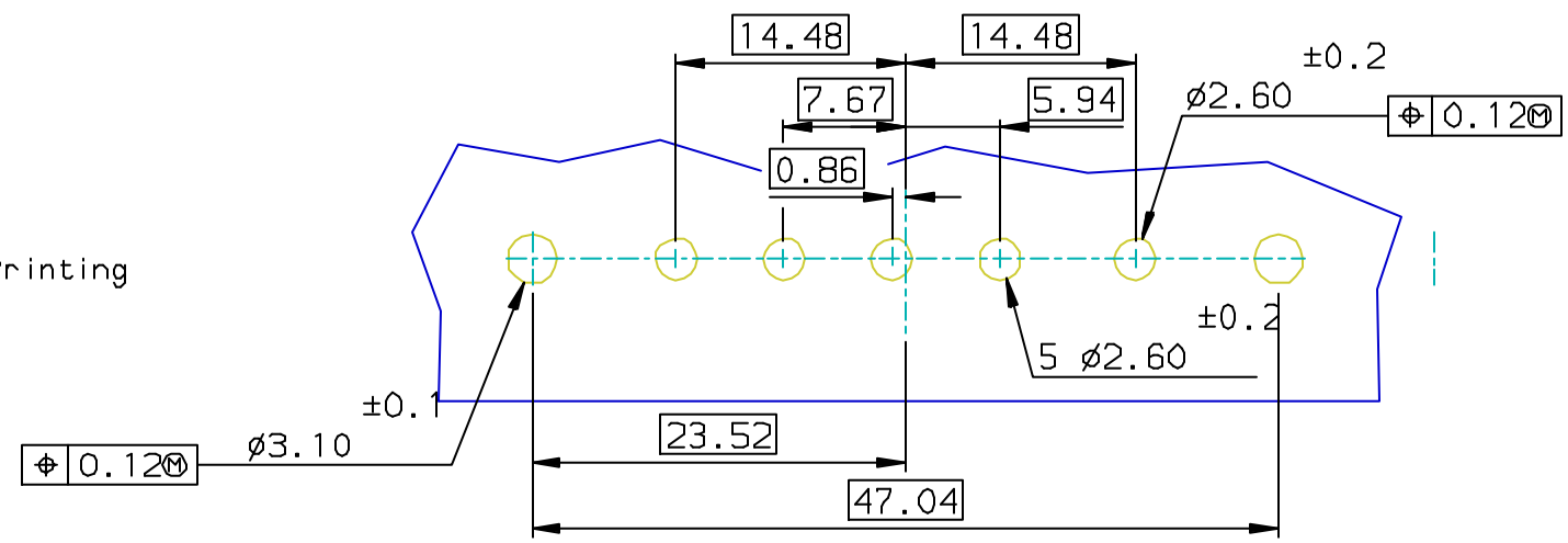
PC CARD DRILLING DIMENSIONS Components side view - Thickness 1.60mm
