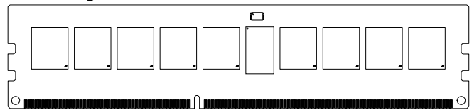
Figure 2: 240-Pin RDIMM (MO-269 R/C B1)
