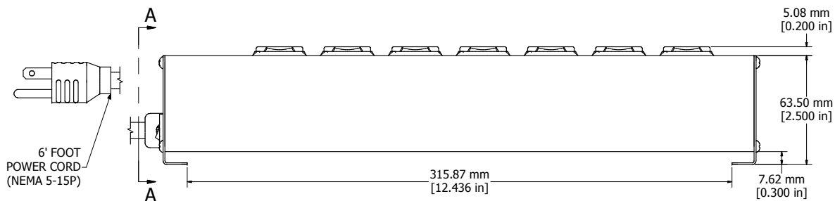
ASSEMBLY - VIEW FROM SIDE
