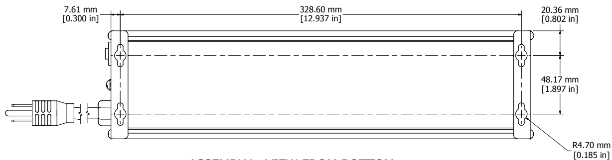
ASSEMBLY - VIEW FROM BOTTOM
