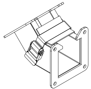
ISOMETRIV VIEW
