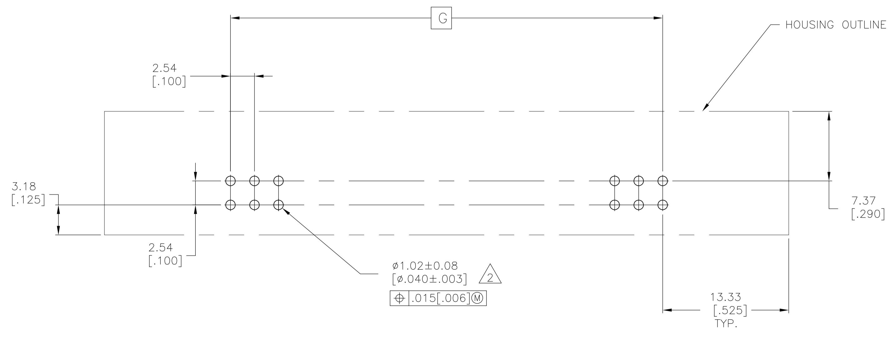
RECOMMENDED PCB HOLE LAYOUT
